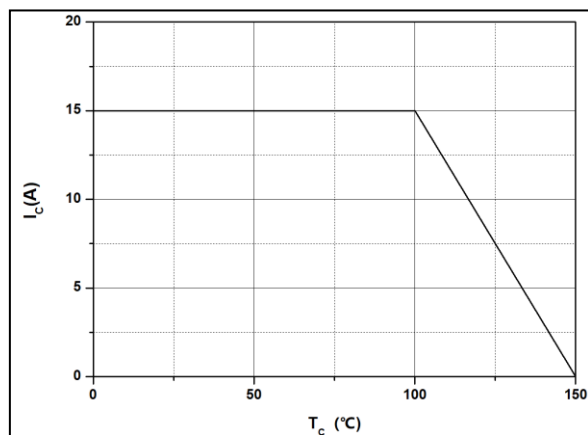
Collector Current VS Case temperature (typical)
