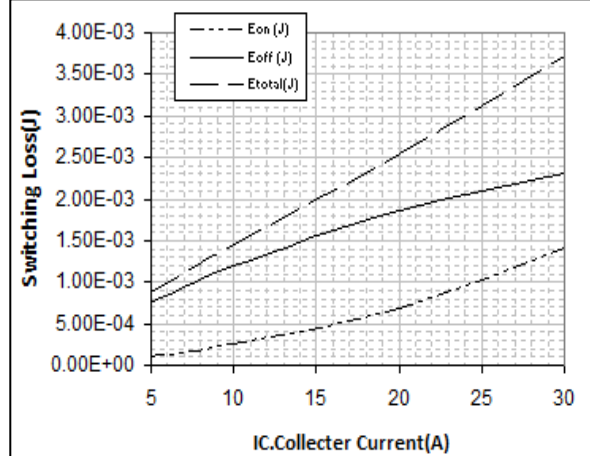
Inverter/Brake-Chopper IGBT Switching Loss vs. I_C(25^{\circ}\text{C})
