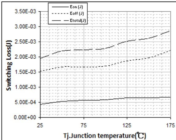
Inverter/Brake-Chopper IGBT Switching Loss vs. T_j
