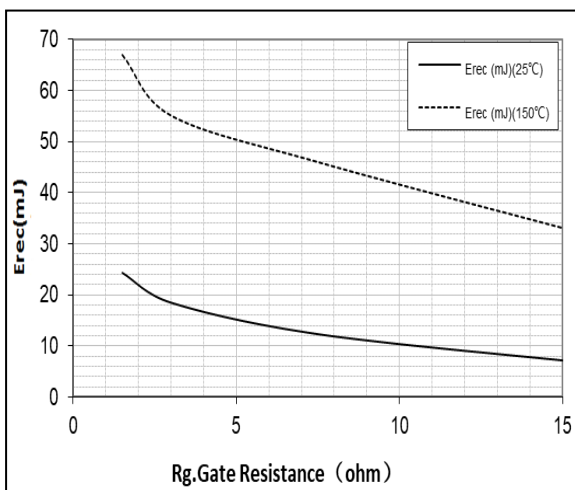
Switching loss Diode, E_{rec} vs. R_G ( I_F=600A , V_{CE}=600V )
